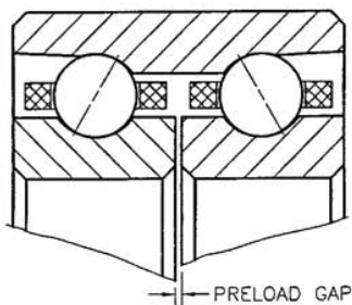
M—TYPE SUPERDUPLEX BACK-TO-BACK
