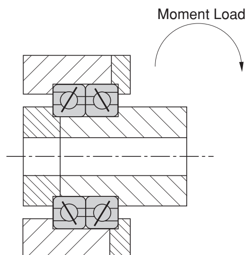
B-Type Configuration
