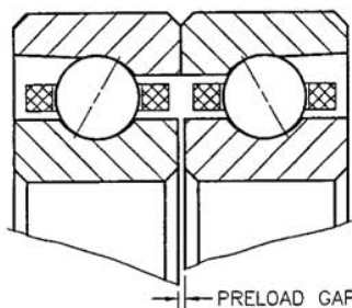
B—TYPE DUPLEX BACK-TO-BACK (DB)
