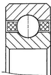
C—TYPE (RADIAL CONTACT)
